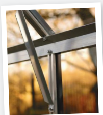
CANTILEVER BRACES
